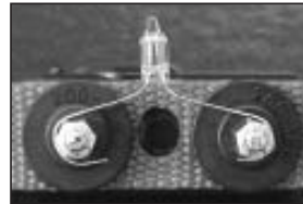
Test Light on Receiver Contact Points
